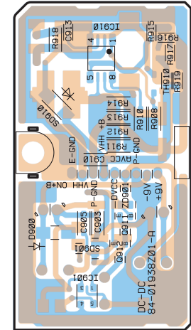
BOX P.W.Board (Foil Side View)
