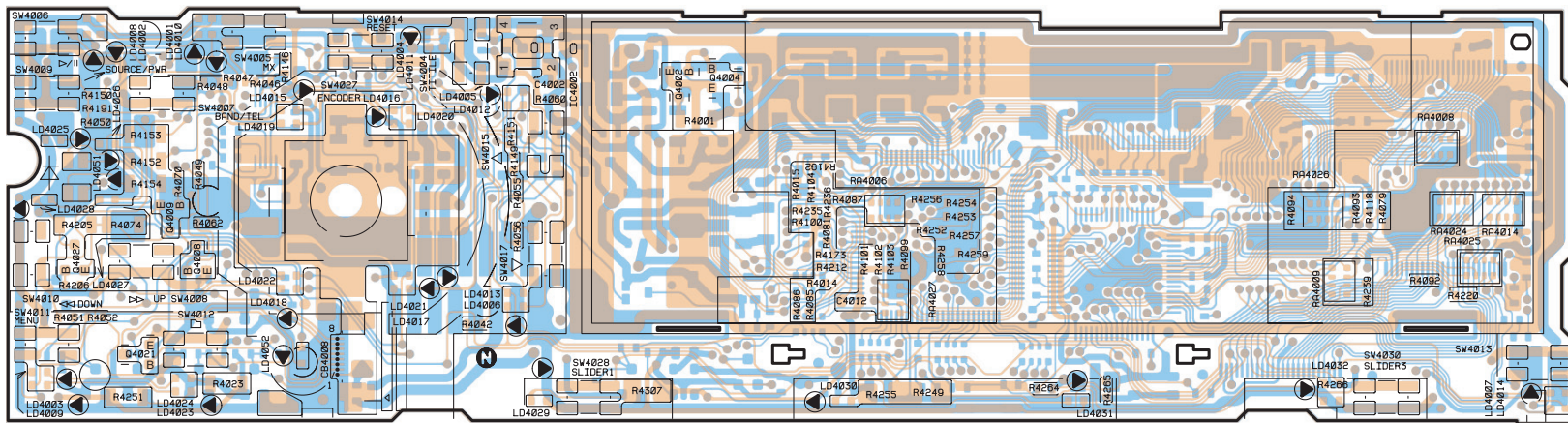
FRONT P.W.Board (Component Side View)
