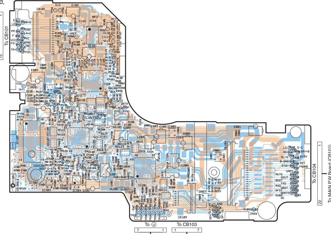
DP-S MAIN P.W.Board (Foil Side View)
