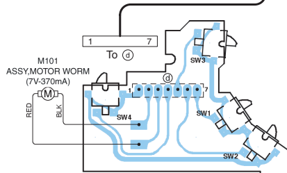
DP-S Switch P.W.Board (Foil Side View)
