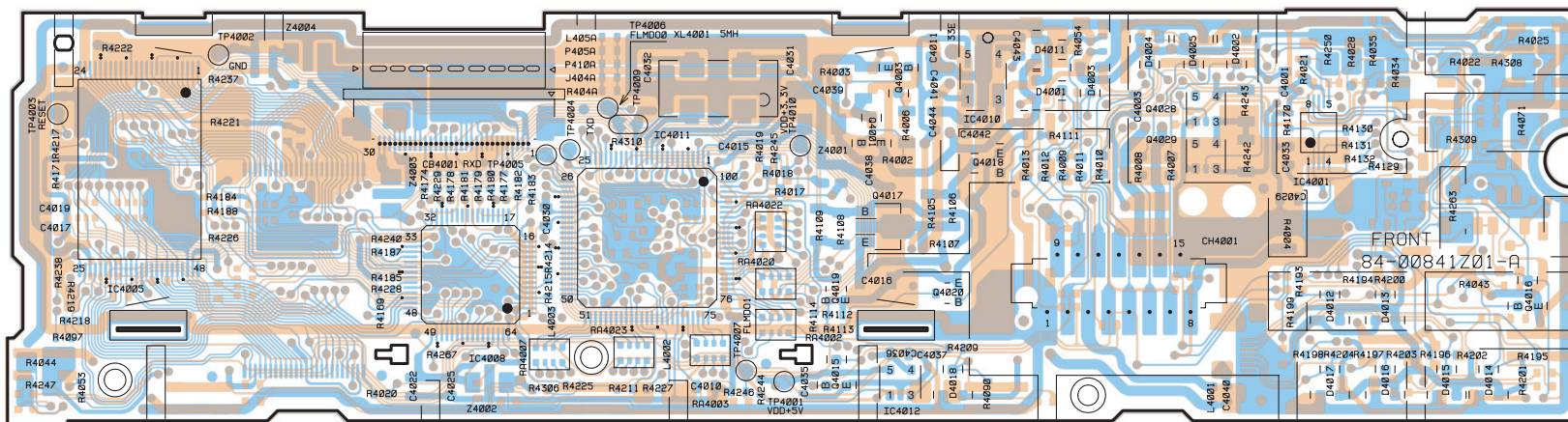
FRONT P.W.Board (Foil Side View)
