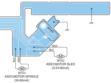
FPC,CONT P.W.Board (Foil Side View)
