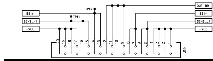
B-Right Channel Amplifier (AB7-2.1)
