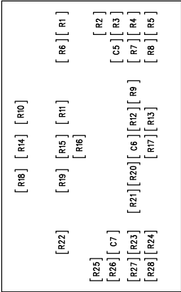
SILKSCREEN BOTTOM
