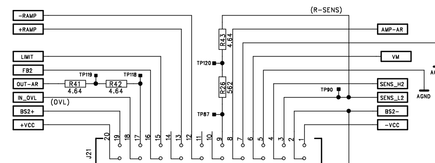
A-Right Channel - Linear Driver (ABLD.1)
