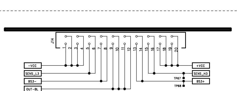
B-Left Channel Amplifier (AB7-2.1)
