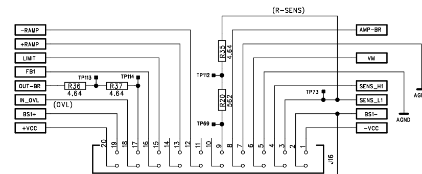
B-Right Channel - Linear Driver (ABLD.1)
