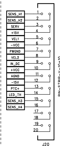
TEST Connector
