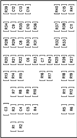
SILKSCREEN BOTTOM
