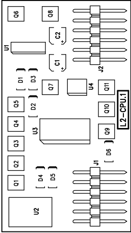
SILKSCREEN TOP
