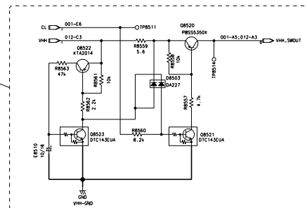
VHH SW &amp; Protection
