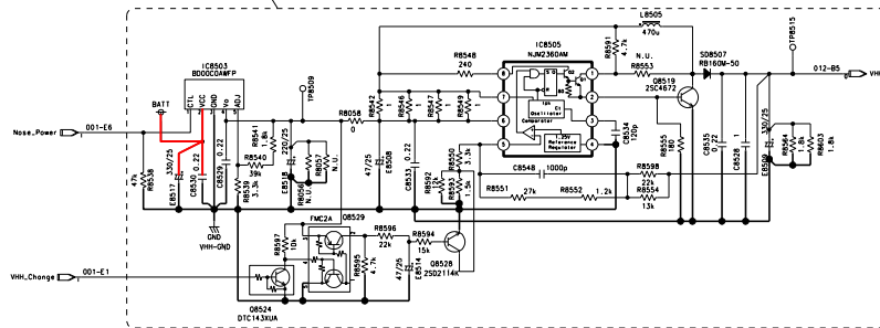
VHH 15V Circuit
