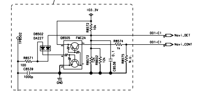
Navi-Control
