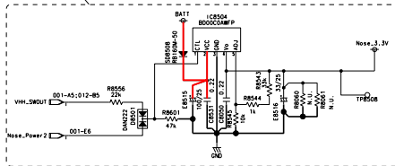
FRONT3.3V Circuit
