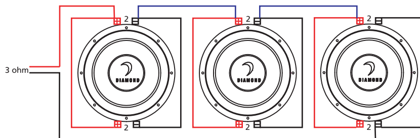
(3) D2's Series-Parallel 3 Ohm Load
