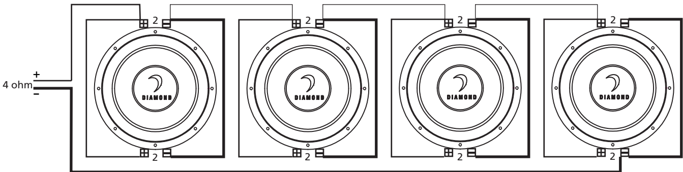
(4) D2's Series-Parallel 4 Ohm Load
