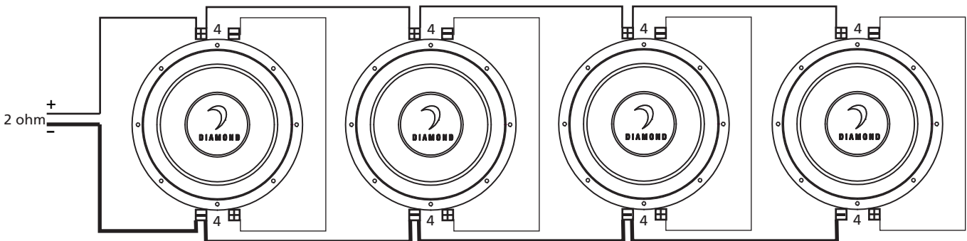
(4) D4's Series-Parallel 2 Ohm Load
