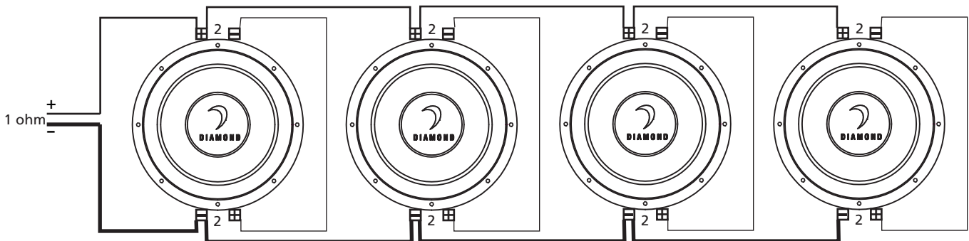
(4) D2's Series-Parallel 1 Ohm Load
