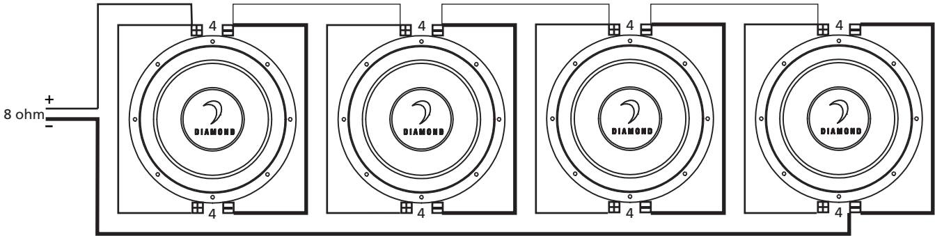
(4) D4's Series-Parallel 8 Ohm Load
