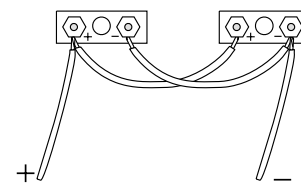
Figure 2. Series connection
