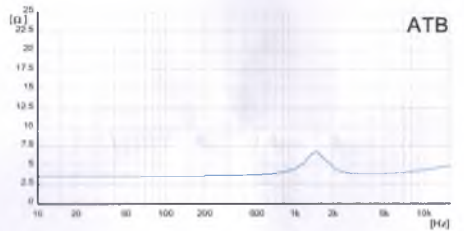
Impedance
