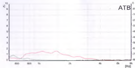
Harmonic Distortion [1W/1m]
