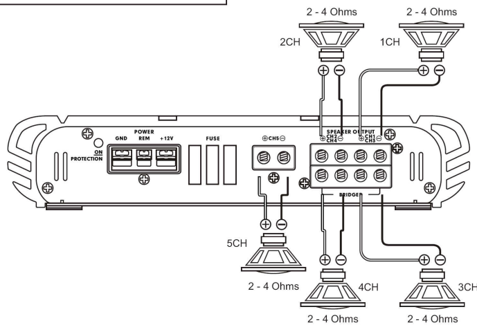
4 SPEAKER + 1 SUBWOOFER
